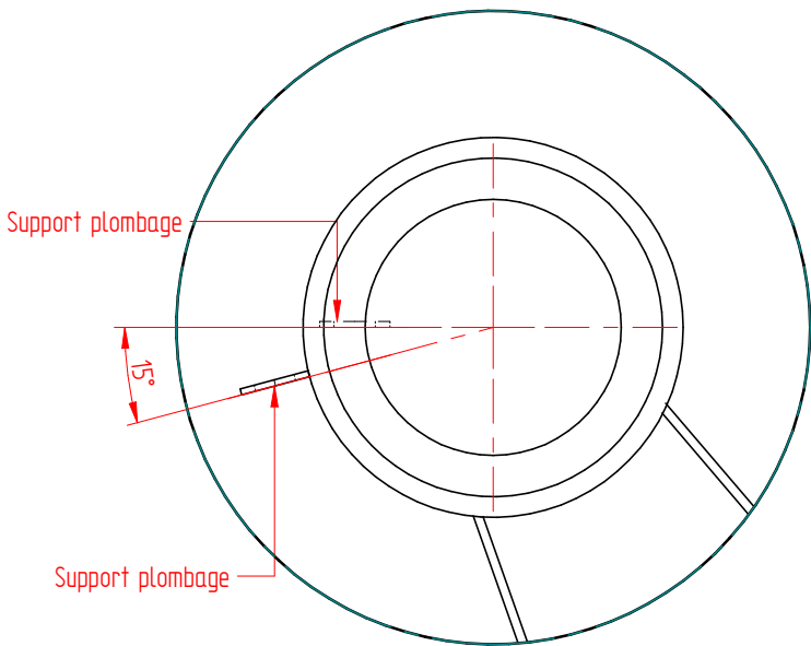
DETAIL B
