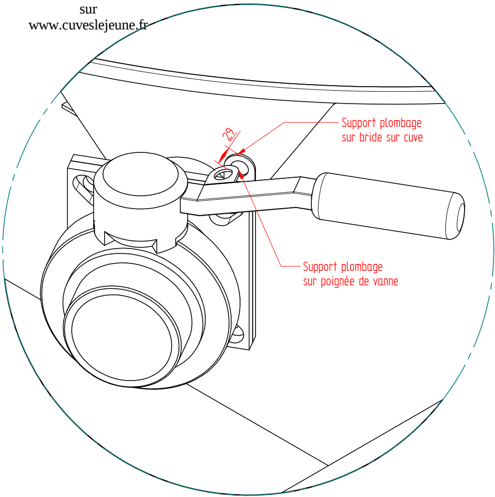
DETAIL C
